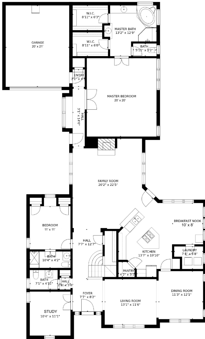
FLOOR 1
